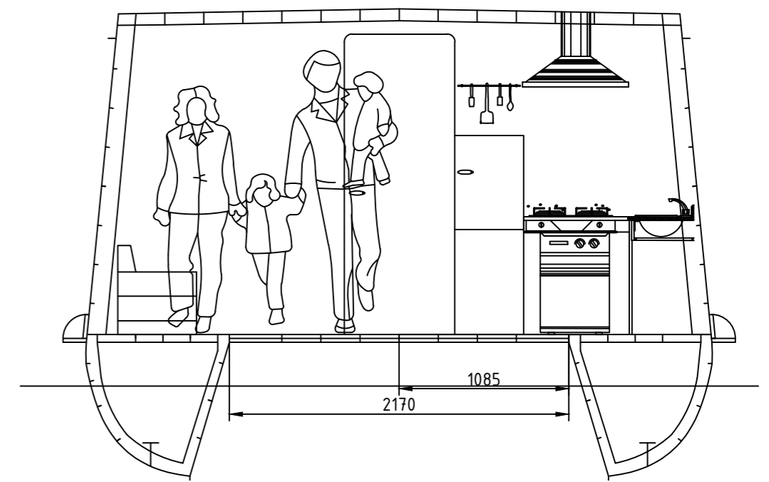
MIDSHIP SECTION
